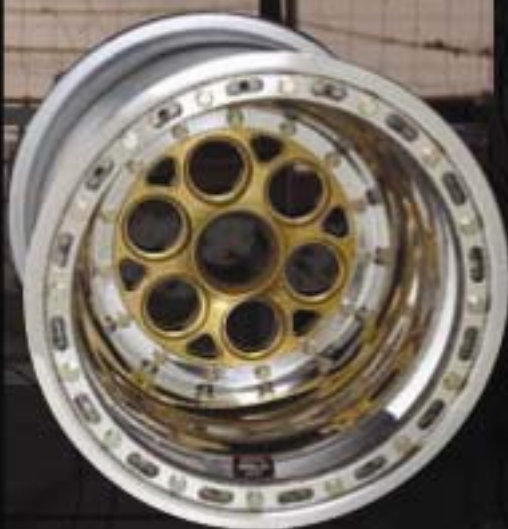
735-51425 15" Magnum Sprint Spline Bead-Loc™ Design Patent Pending
